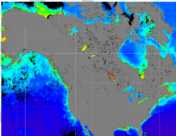
Figure 6: Example of NASA MODIS imagery.
